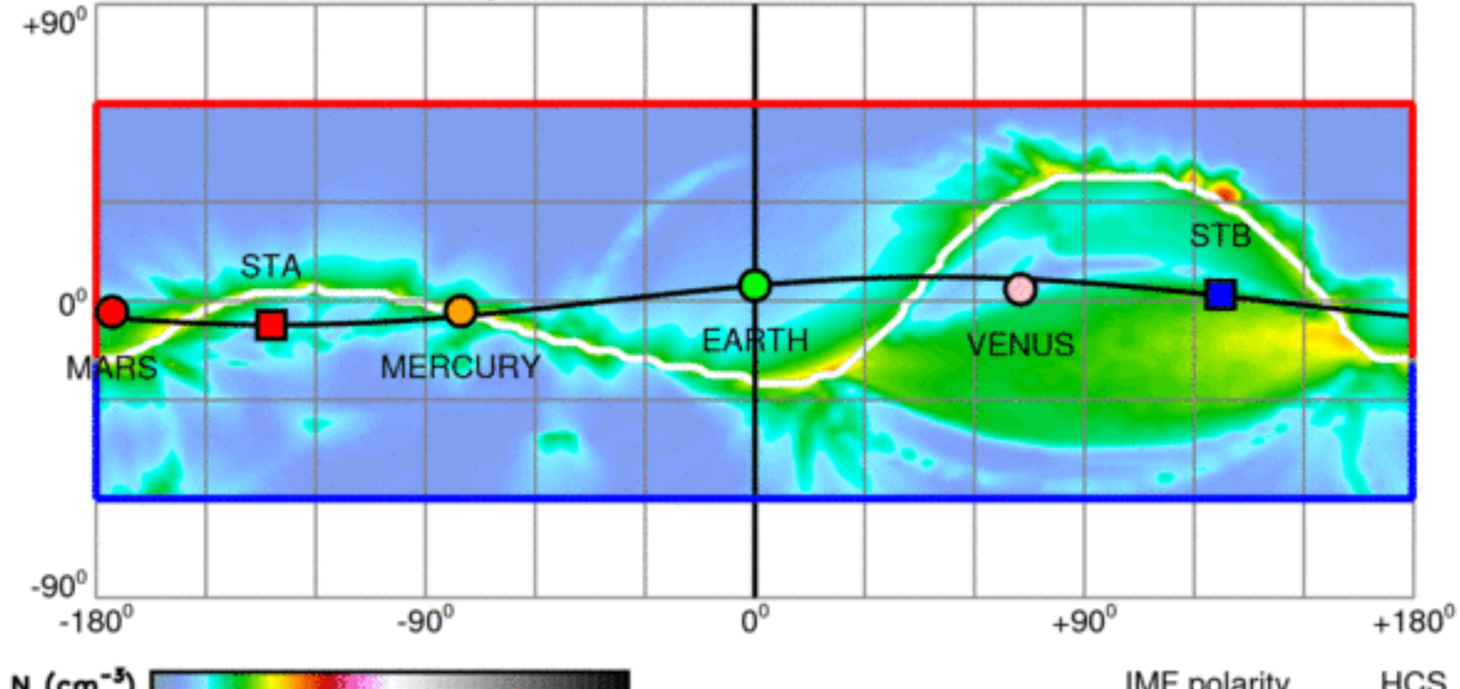
(b) Solar wind number density
