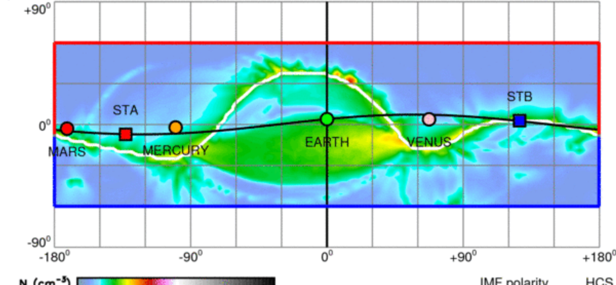
(b) Solar wind number density
