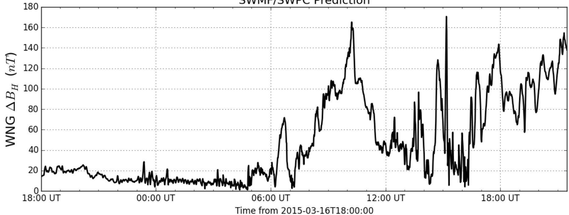
SWMF/SWPC Prediction
