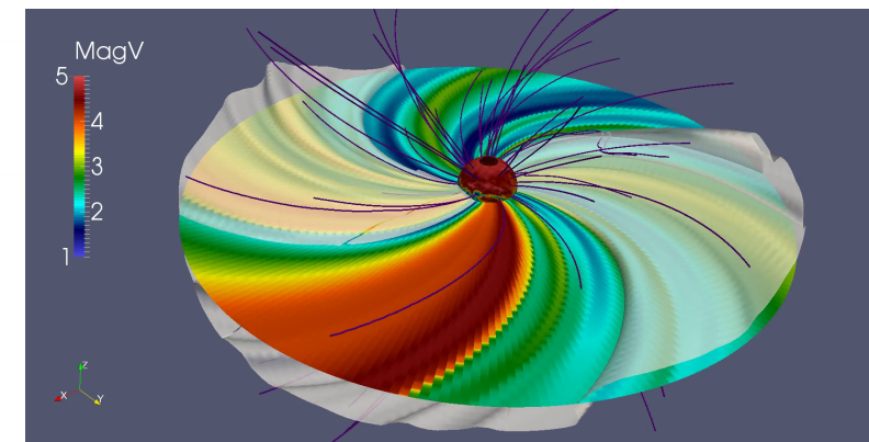
Inner heliosphere
