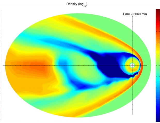
Saturn magnetosphere
