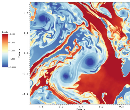
Hydro Kelvin-Helmholtz Elapsed Time: 5.05 (s)
