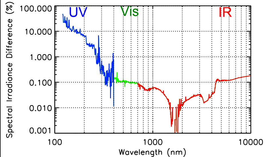
Spectral Solar Irradiance (SSI): SMax vs. SMin
