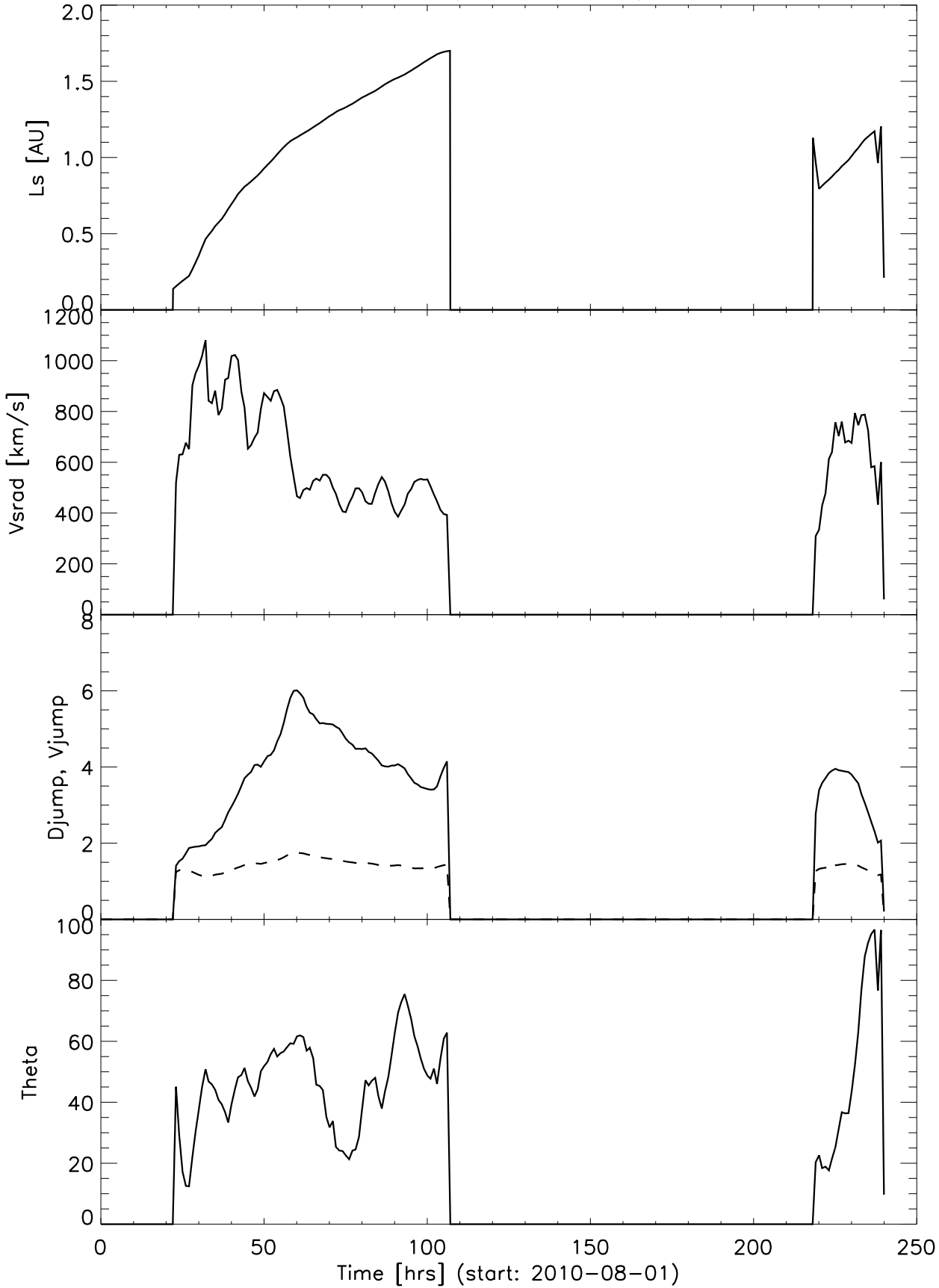
Earth (2010-08-01)
