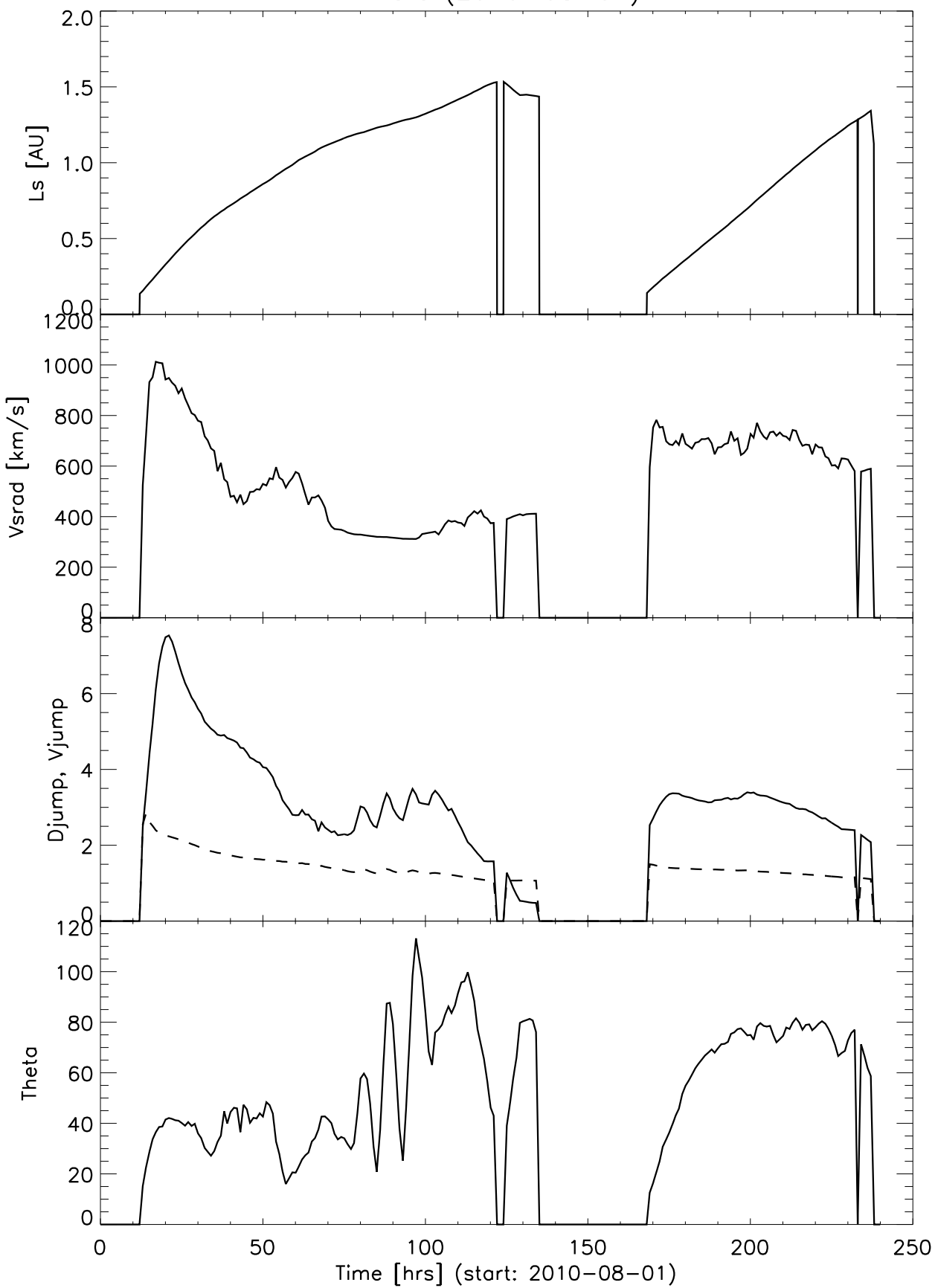
Mars (2010-08-01)
