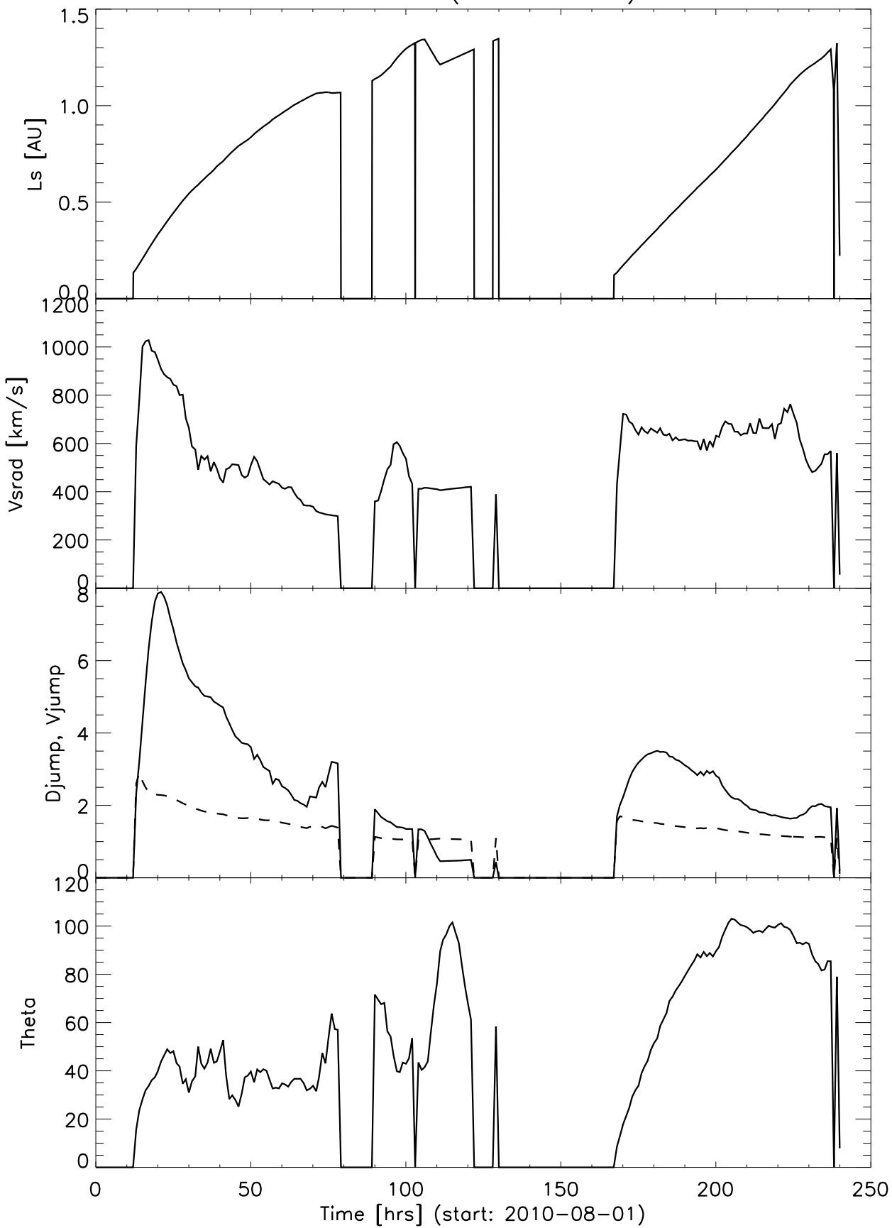
Stereo_B (2010-08-01)
