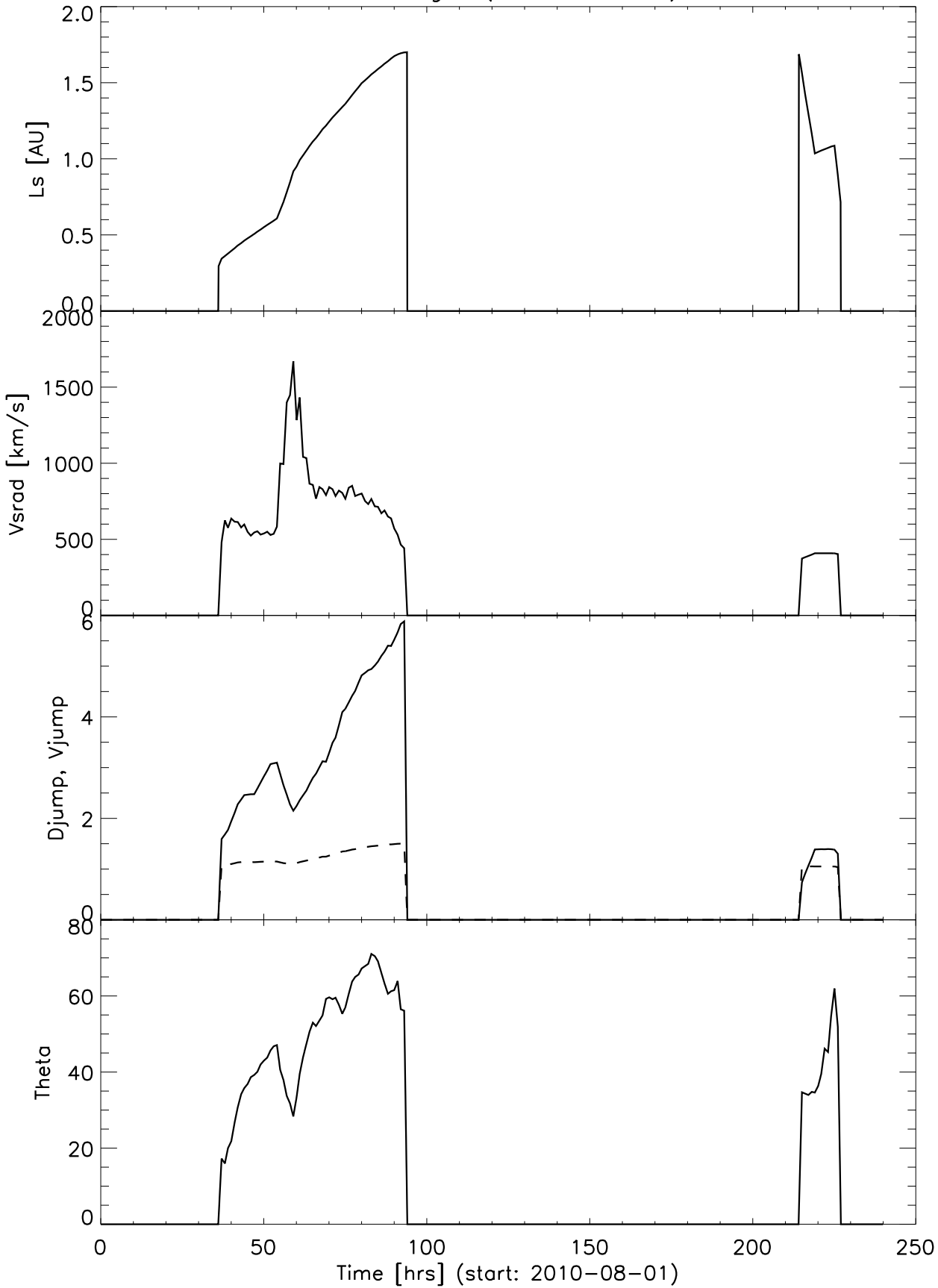
Messenger (2010-08-01)
