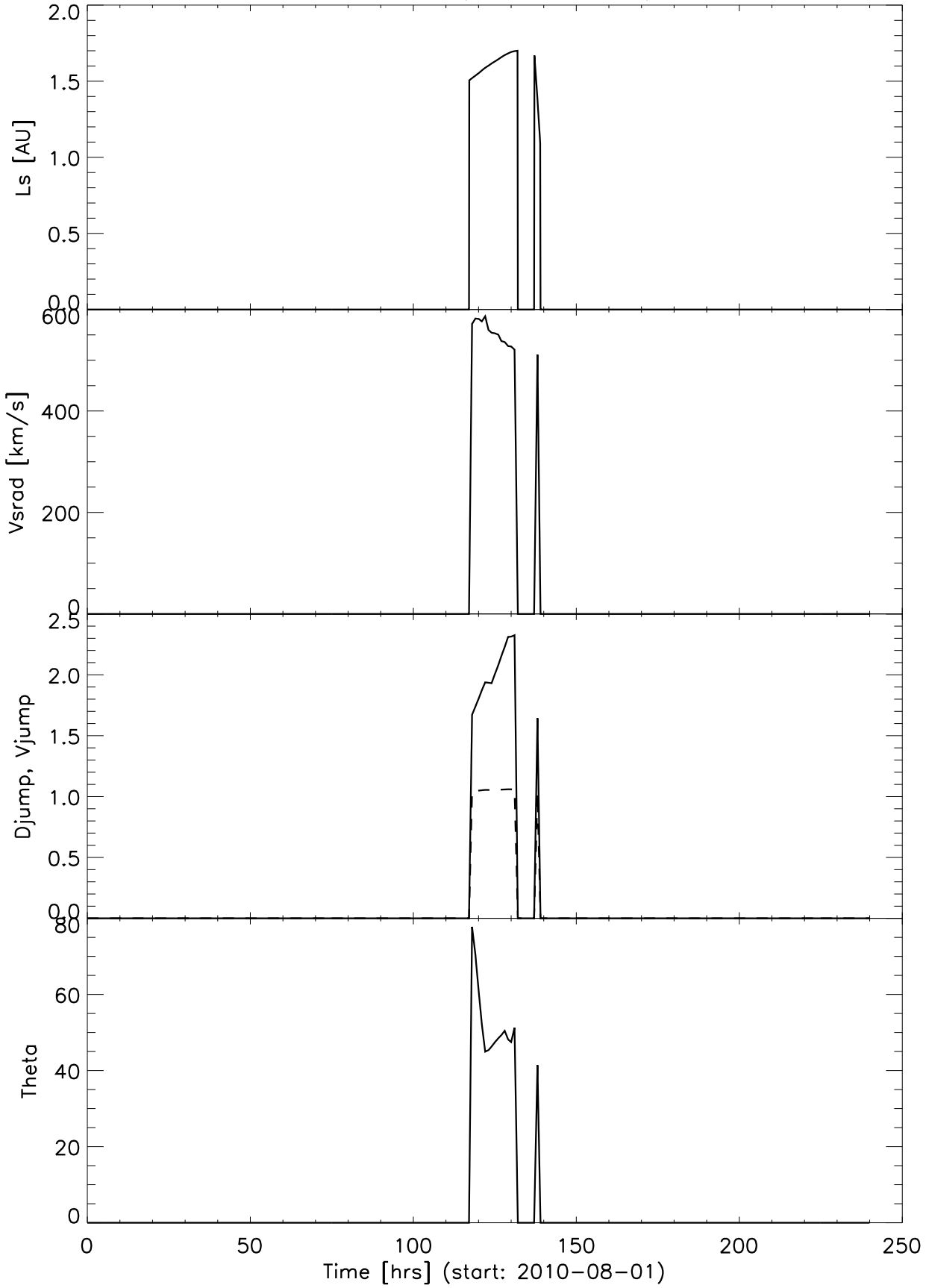
Stereo_A (2010-08-01)
